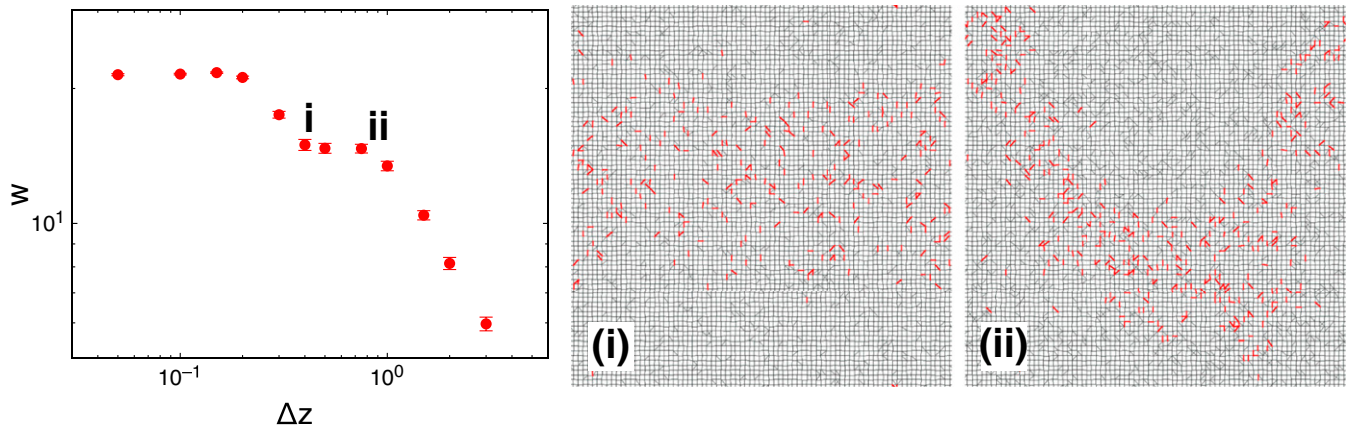
Fig. 3. Crack width vs. \Delta z in random-network simulations with a square geometry. The images are snapshots at the end of the breaking process for two values of \Delta z , labeled i and ii on the plot, illustrating the competition between the intrinsic width and the meandering of a crack. The intrinsic crack width is initially the size of the sample and then decreases with increasing \Delta z . Image (i) shows when the w has first decreased to a second plateau value. As \Delta z increases further, the intrinsic width decreases and becomes comparable to the meandering width of the crack. Image (ii), at the other end of the plateau, shows a meandering crack with a smaller intrinsic width. At larger \Delta z , the entire width of the crack decreases.
